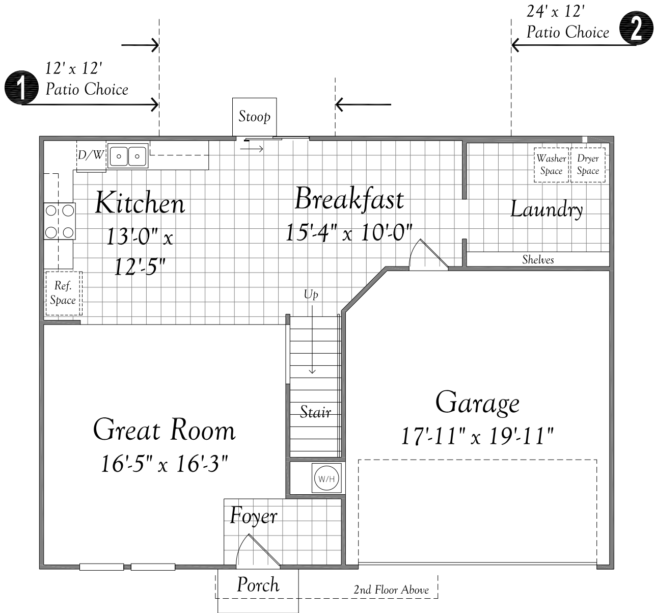
First Floor Country Kitchen
