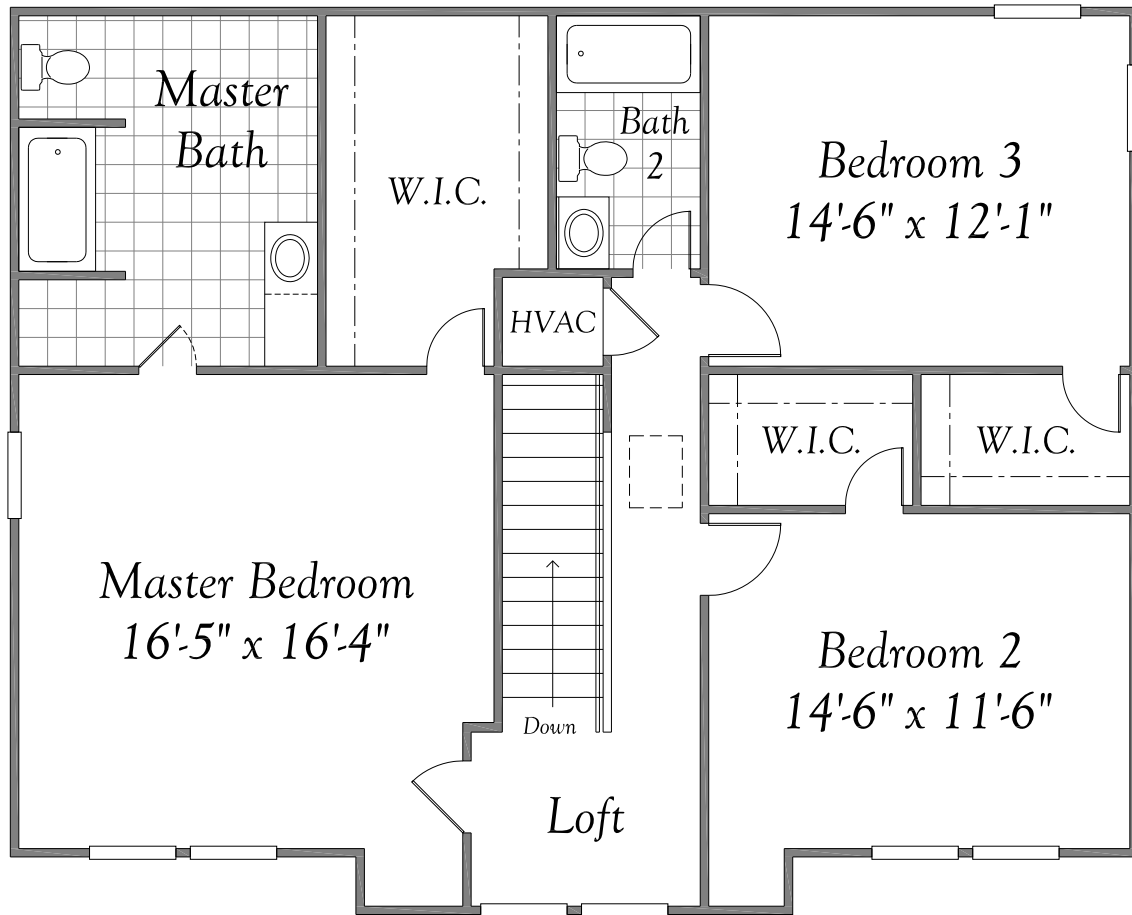
Second Floor Three Bedrooms with Loft
