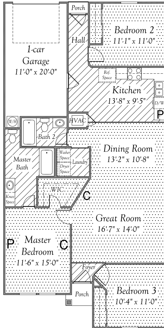
Floor Plan Country Kitchen
